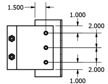
SECTION D-D SCALE 3/16
