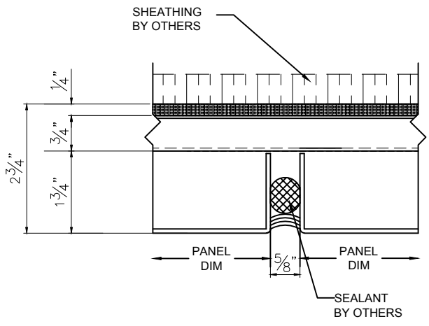
02 XX VERTICAL JOINT DETAIL BPS2 XX SCALE: NONE
